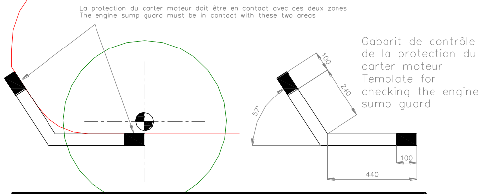
Dessin/Drawing 285-1
